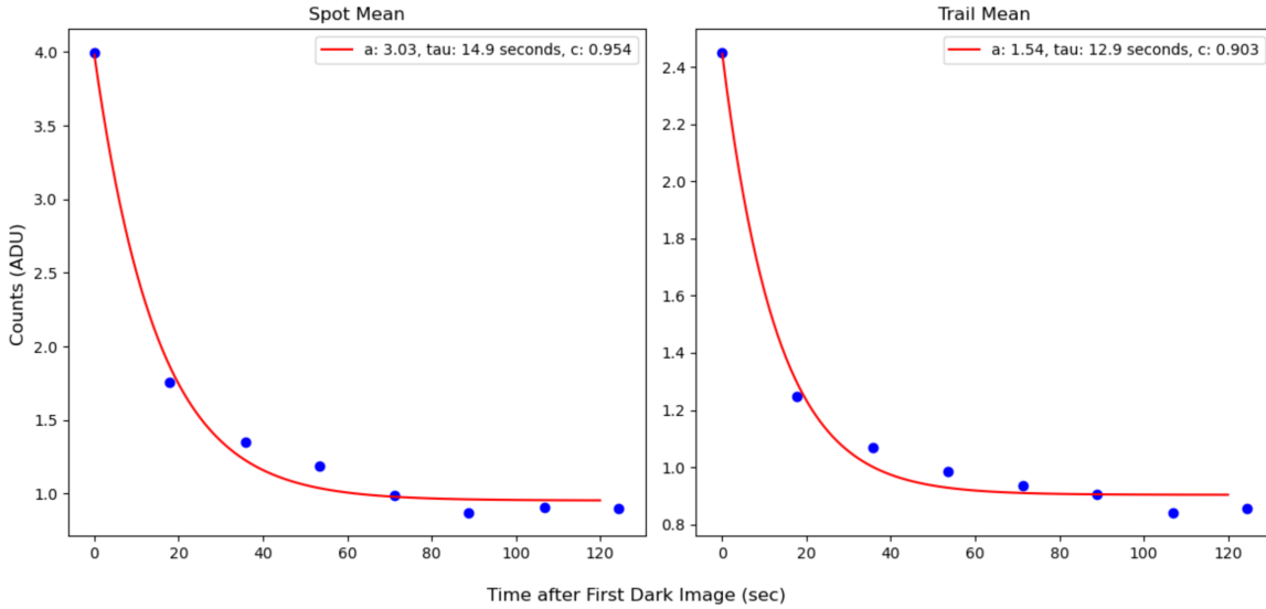
FIGURE 6: The decay of the persistence with consecutive dark images. The blue points are the measured average counts of the spot (left) and trail (right). The red line shows the model fit with the parameters shown in the upper right.
