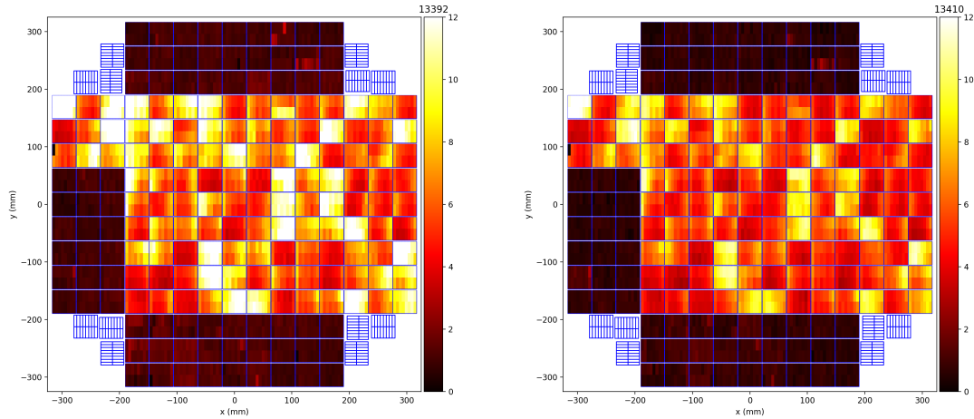
FIGURE 4: Full Focal plane images with amplifier level resolution comparing a subsequent dark image with nominal parallel clock swing voltages (left; Run 13392) and one with a slightly higher parallel clock swing voltage (right; Run 13410).
