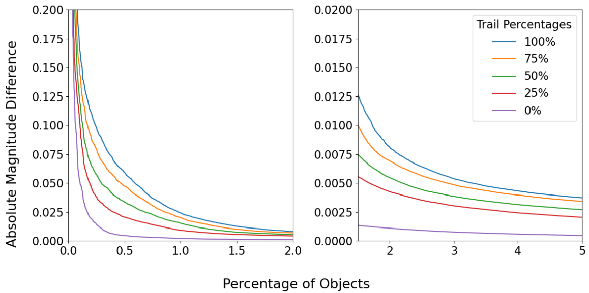
FIGURE 11: Plots showing the cumulation percentage of affected objects when compared to all objects from the 68 images with all the trail scenarios. The left plot highlights the percentage of the most affected objects. The right plot zooms into the area where the cumulation trend levels out.
