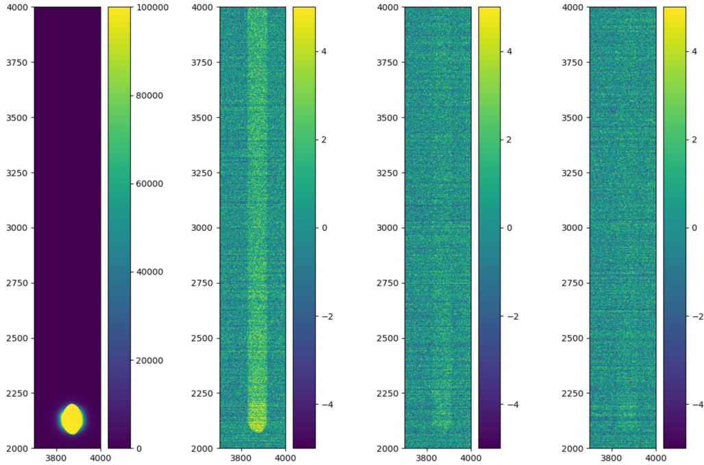
FIGURE 5: Similar to Figure 1 but with the pinhole filter. This shows the initial flash and the spot (left) and the dark images that followed.
