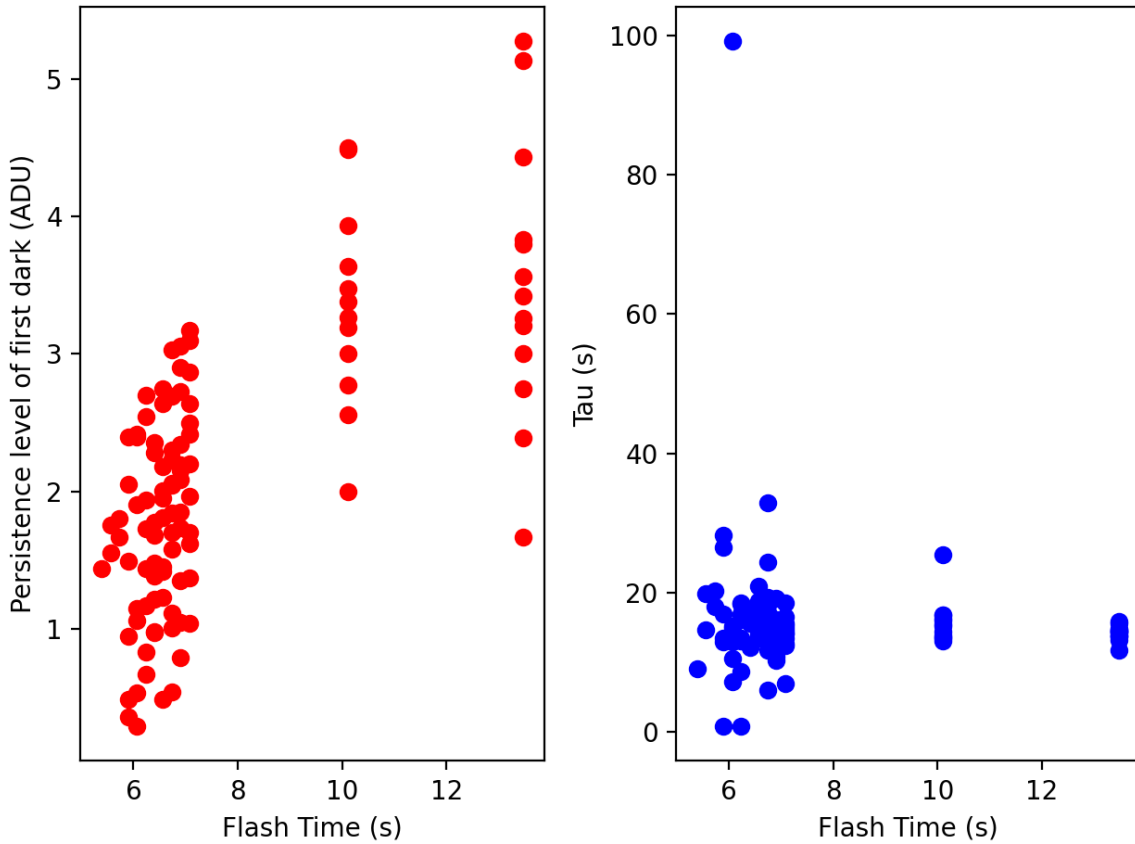
FIGURE 7: The relationship between the duration of the LED flash (a proxy for the brightness of a saturated source) and amplitude (left) and tau (right) for the spot. Each point represents the measured tau and amplitude values of a single sensor from a single exposure that displayed persistence. The amplitude appears to be dependent on the flash time, while tau is invariant and is consistently between 10–20 seconds.
